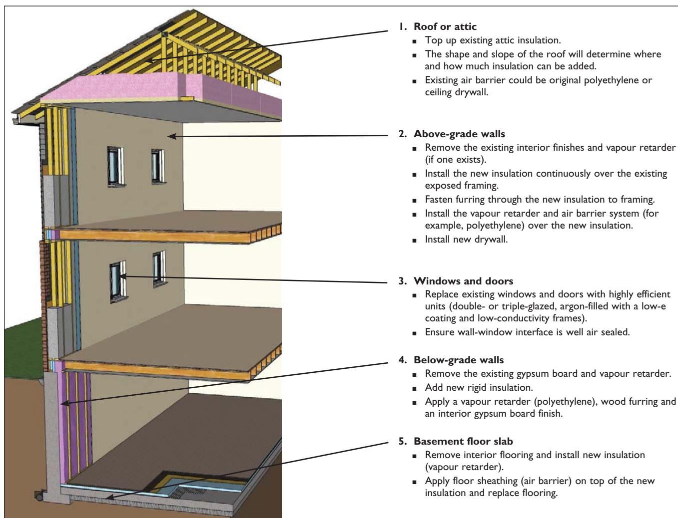
Figure 2 Interior insulation retrofit approach: post-retrofit section
